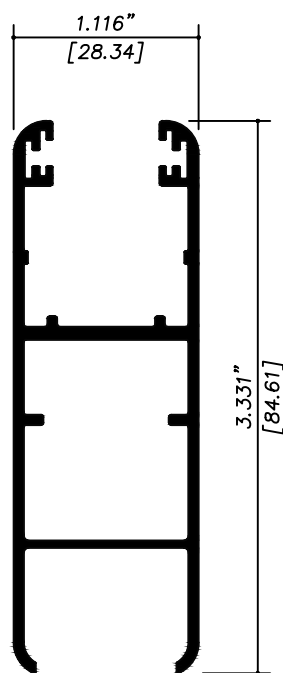
PP42319 HOJA PUERTA DUO
