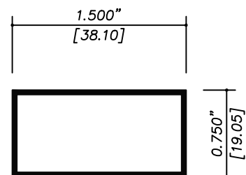
11086 RECTANGULAR 1 1/2 X 3/4"
