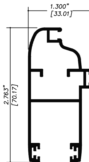
PP4002 MOSQUITERO CURVO
