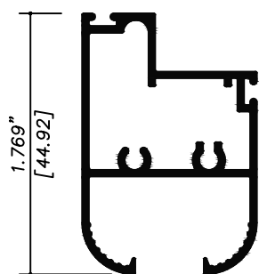
2231 MARCO COLONIAL
