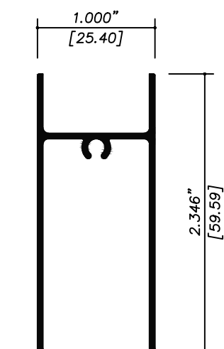
7835D ZOCLO VENTANA DUO
