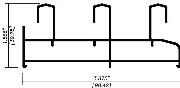
PP4005 RIEL TRIPLE
