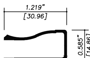
9525 MARCO 1 1/4"
