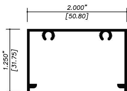
8591 BOLSA LISA
