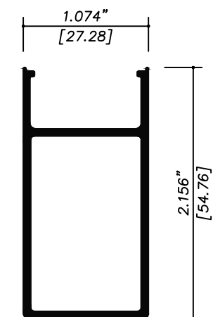
7847D CERCO CHAPA DUO
