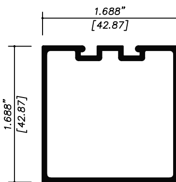
9184 REPATE PUERTA 1 3/4"
