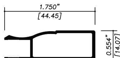
9756 MARCO 1 3/4"
